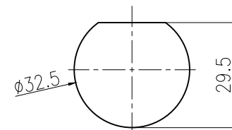
面板安装孔尺寸 mounting hole size on panel
