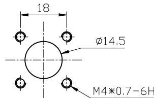
面板安装孔直径 mounting hole size on panel
